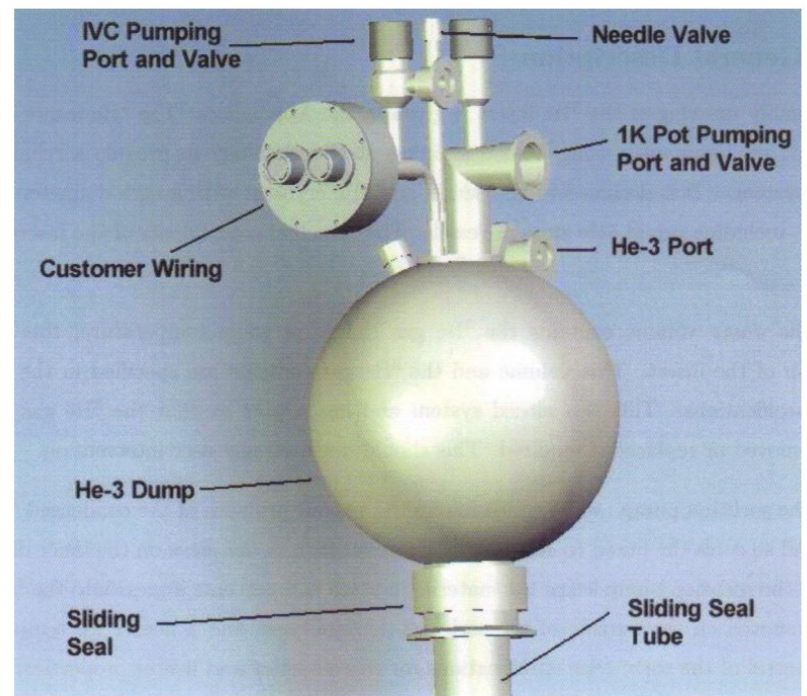
Figure 1: Generic image of the top of a ^3\text{He} insert
