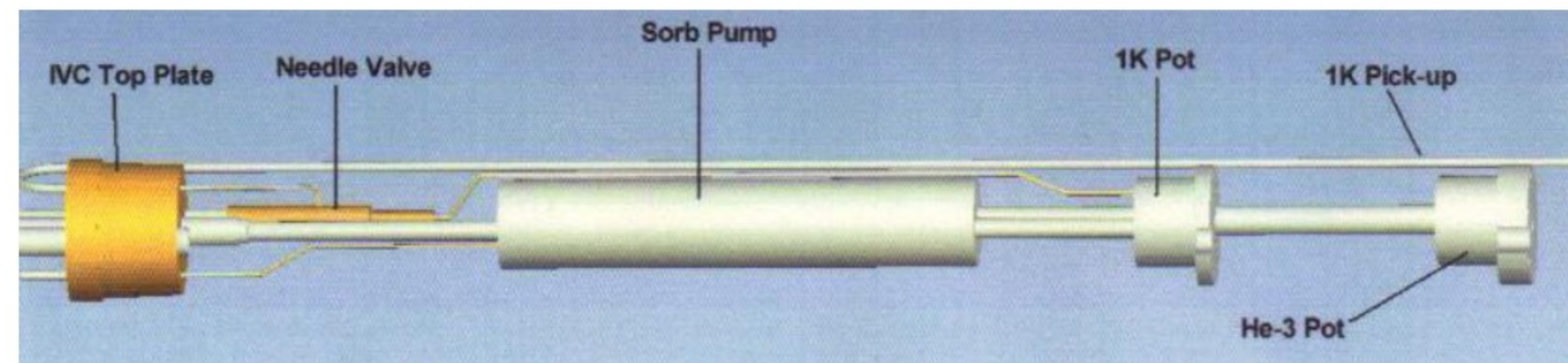
Figure 2: A generic drawing of the low temperature region of a ^3\text{He} system. Some modifications have been made to this system.
